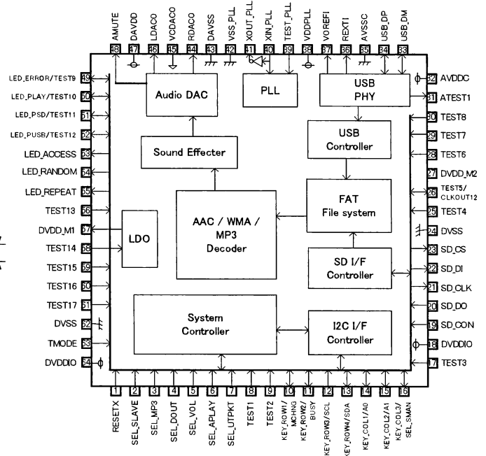
Figure 2. Block diagram
