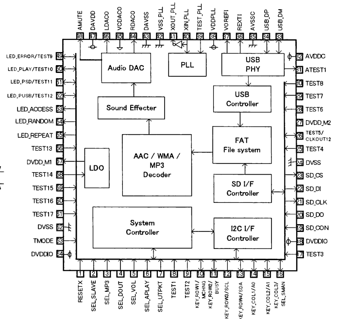
Figure 2. Block diagram
