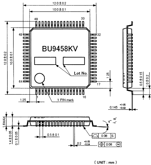
Figure 1. External dimension
